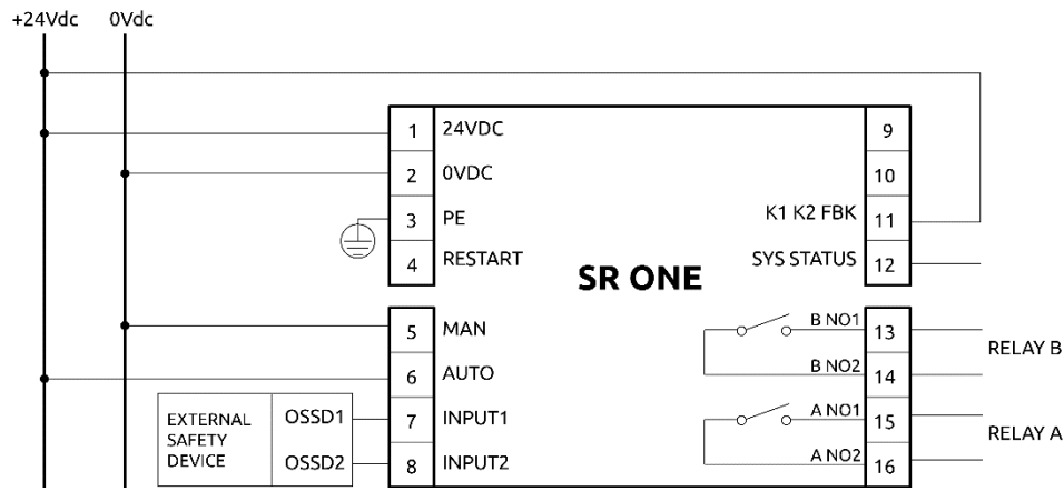
Example of connection of the SR ONE in AUTOMATIC operation
