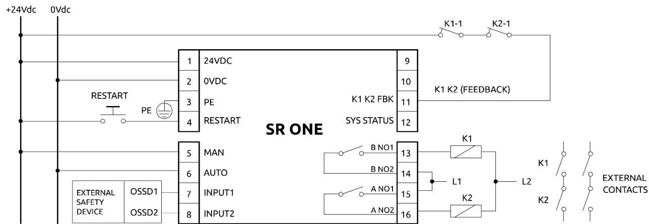
Example of connection of the SR ONE in MANUAL operation with K1 K2 relays
