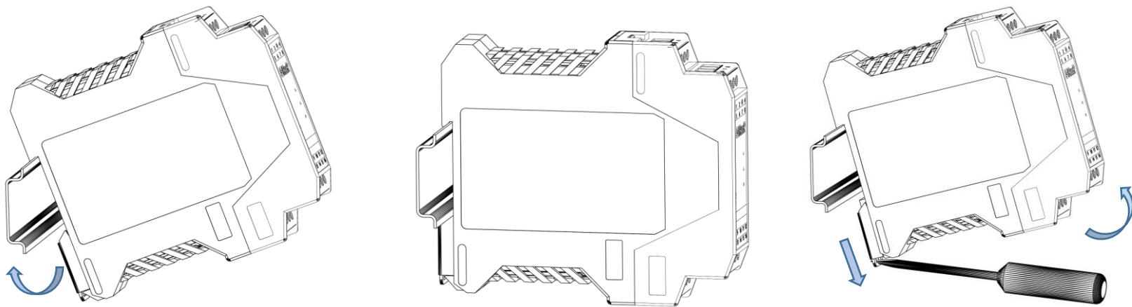
Figure 1 – Montaggio-smontaggio meccanico / Mechanical assembly-disassembly
